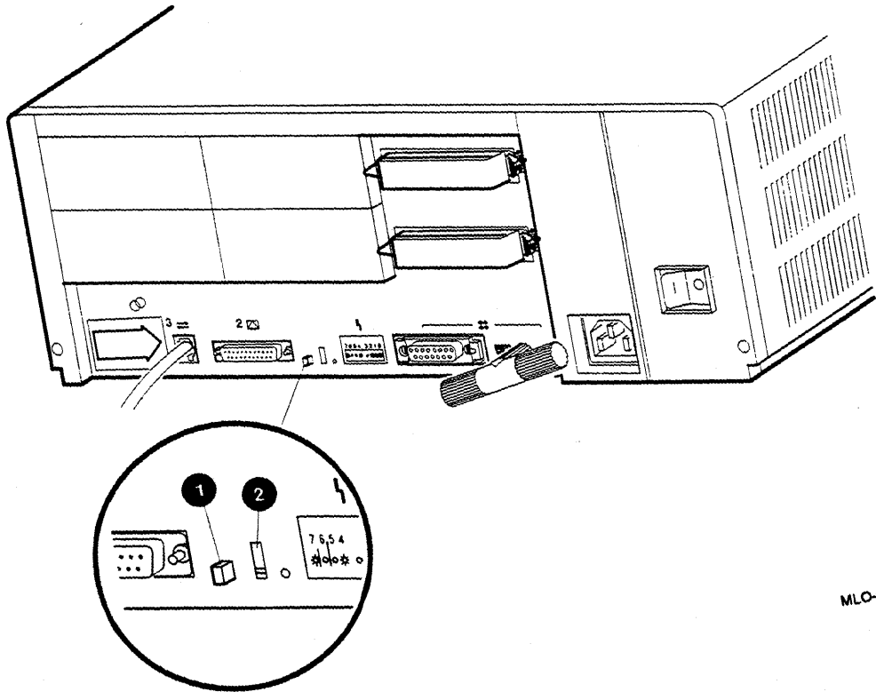
Figure 2-1 Model 85/95 System Halt Button
